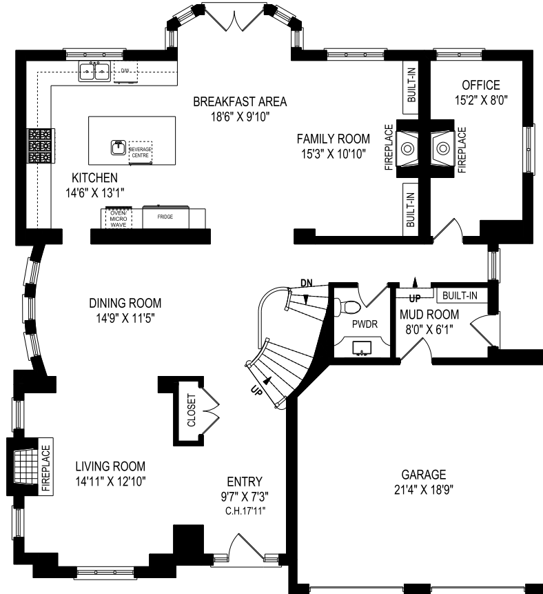
MAIN FLOOR 1651 SQUARE FEET CEILING HEIGHT 9'
