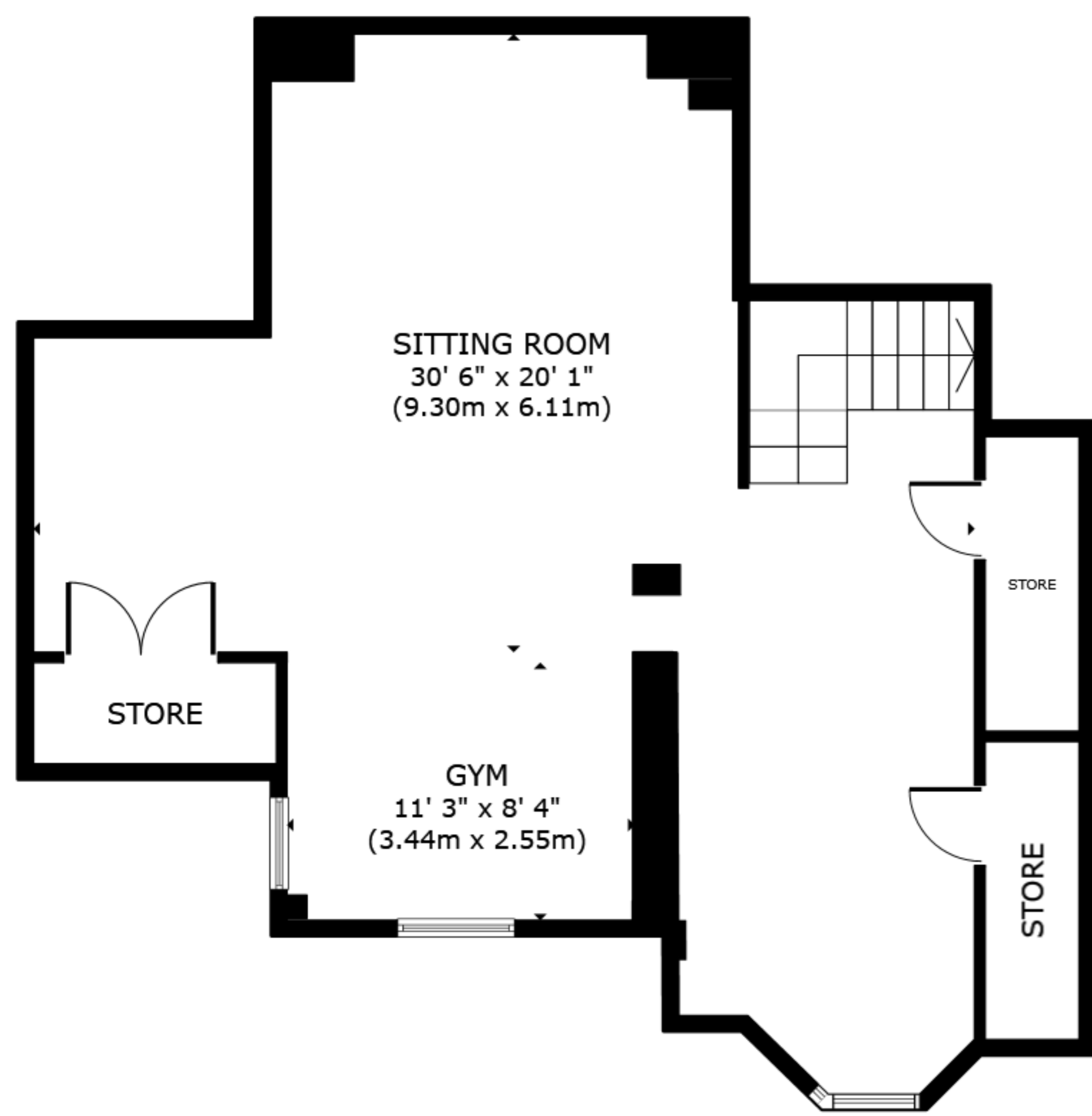
FLOOR 1
