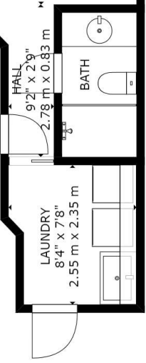
FLOOR 1
