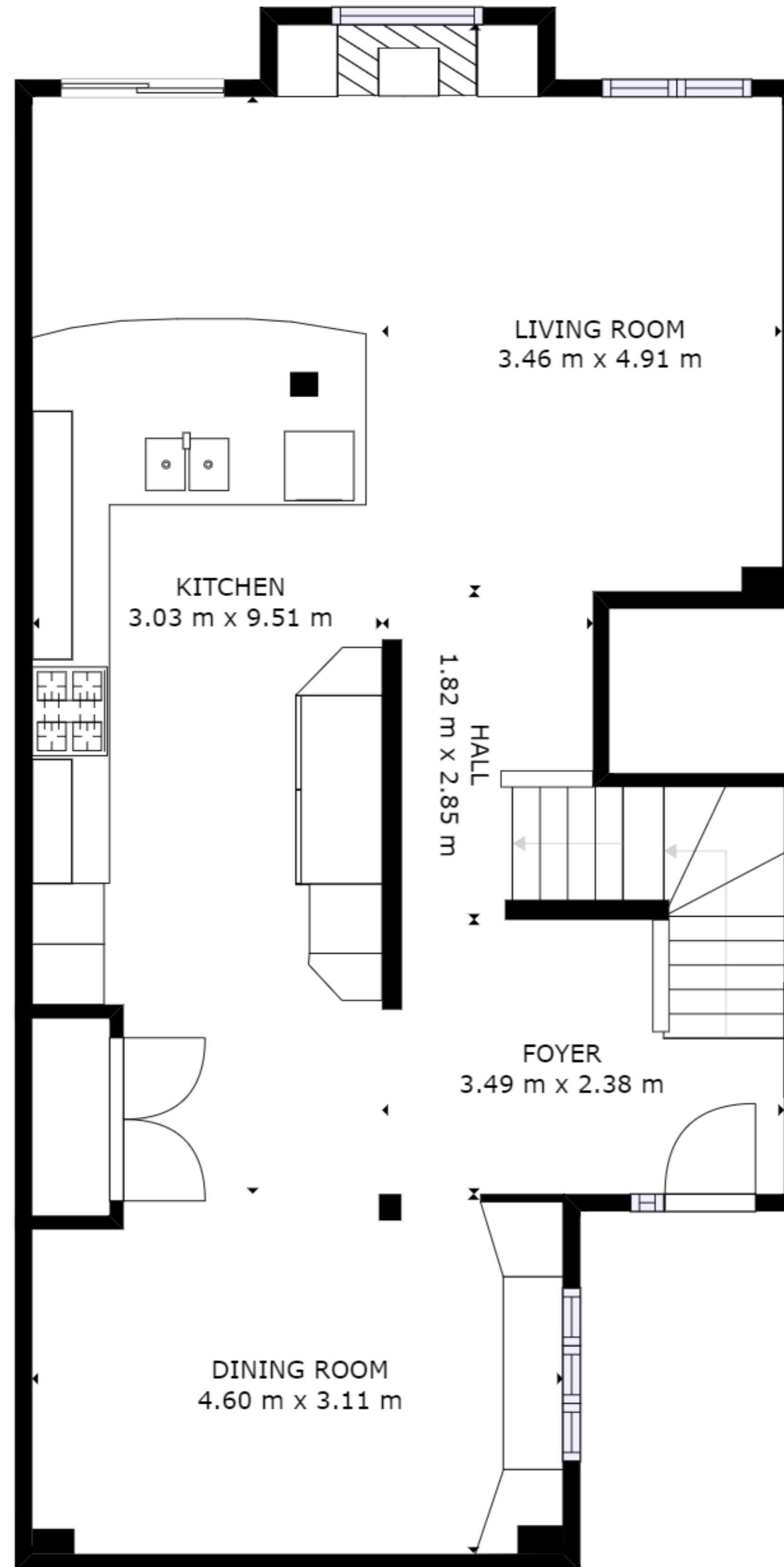
FLOOR 2
