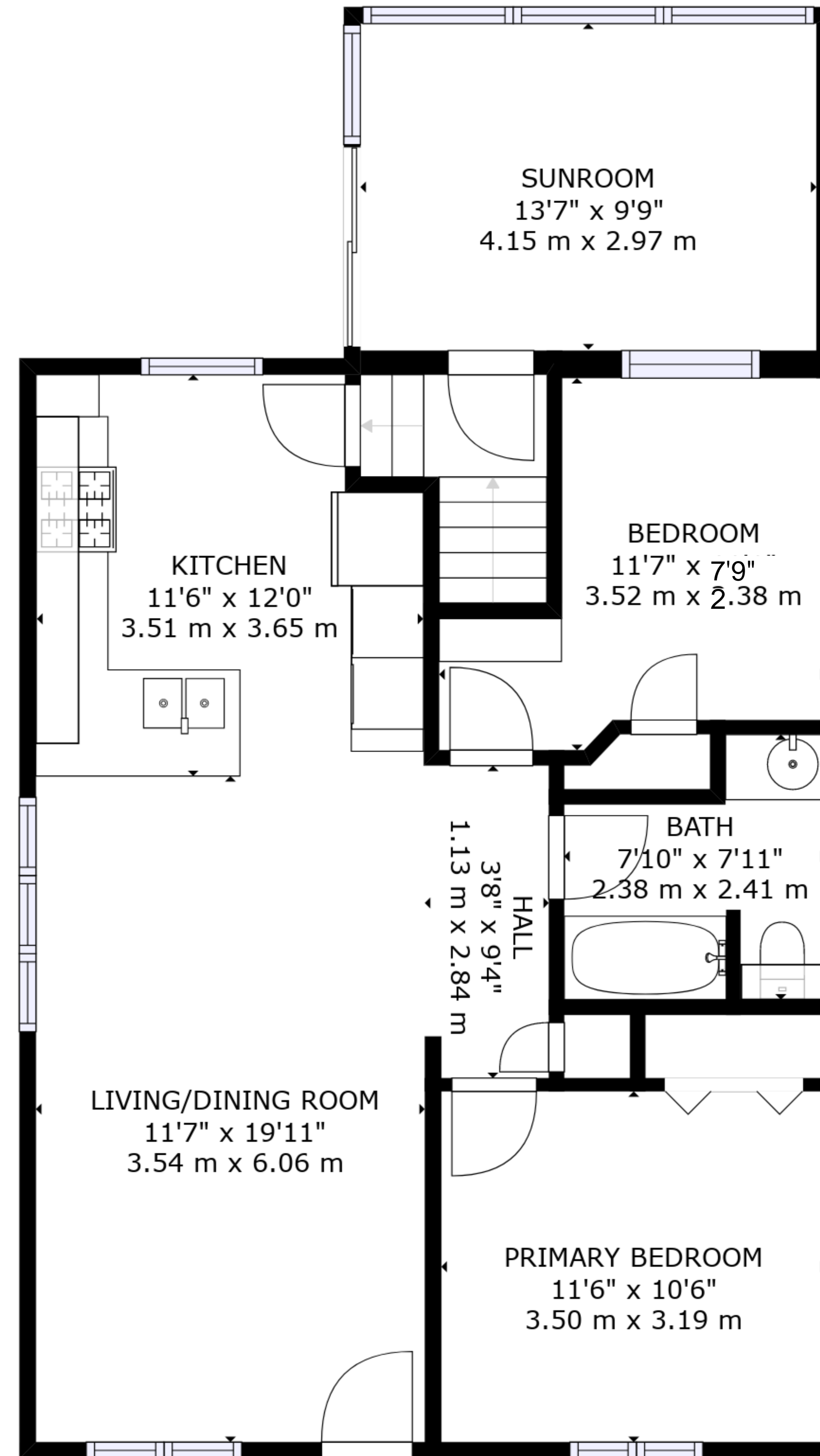
FLOOR 2
