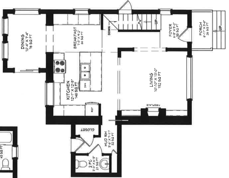
MAIN FLOOR LIVING AREA 786 SQ FT
