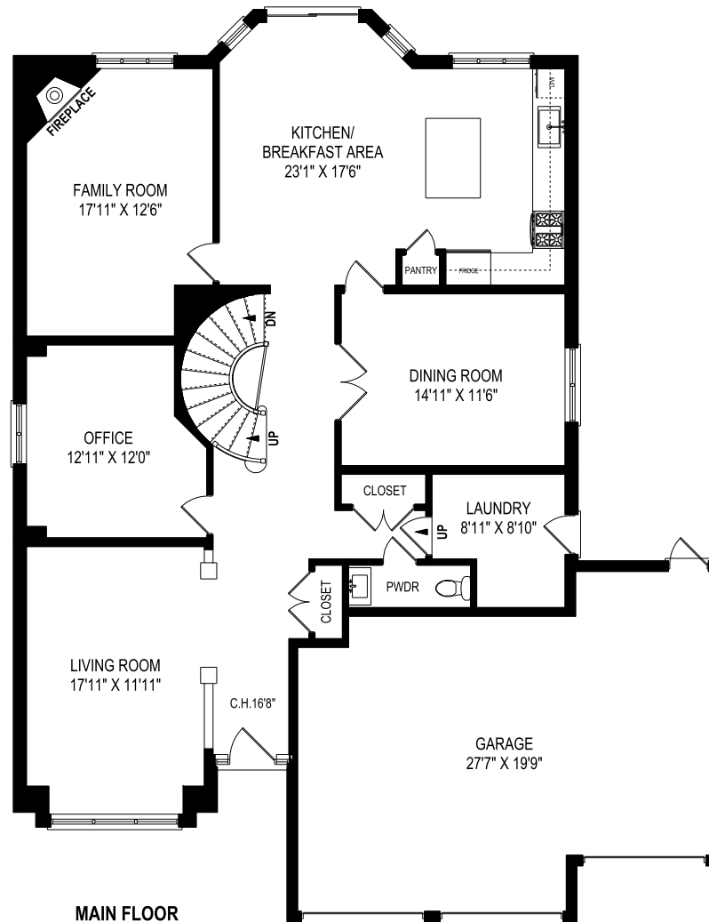
MAIN FLOOR 1706 SQUARE FEET
