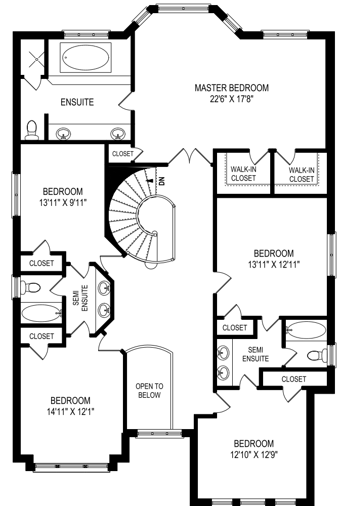
SECOND FLOOR 1947 SQUARE FEET AREA EXCLUDES 49 SQUARE FEET OPEN TO BELOW
