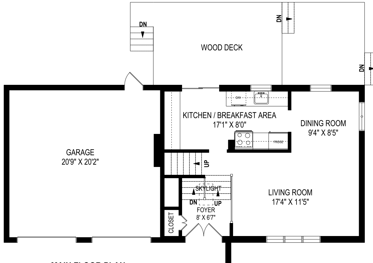
MAIN FLOOR PLAN 610 SQUARE FEET
