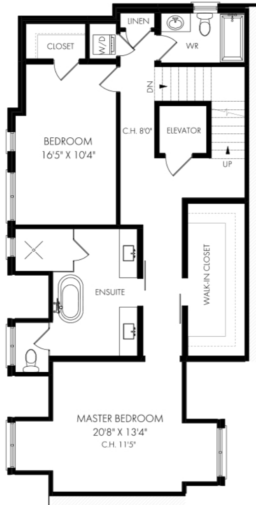
CEILING HEIGHT 8'0" THIRD FLOOR - 1115 SQUARE FEET
