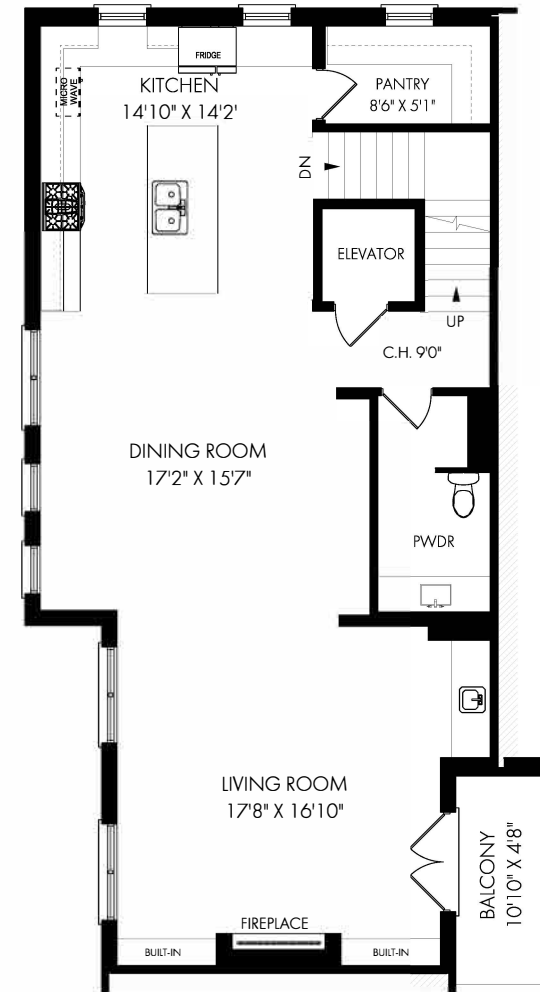
CEILING HEIGHT 9'0" SECOND FLOOR - 1143 SQUARE FEET
