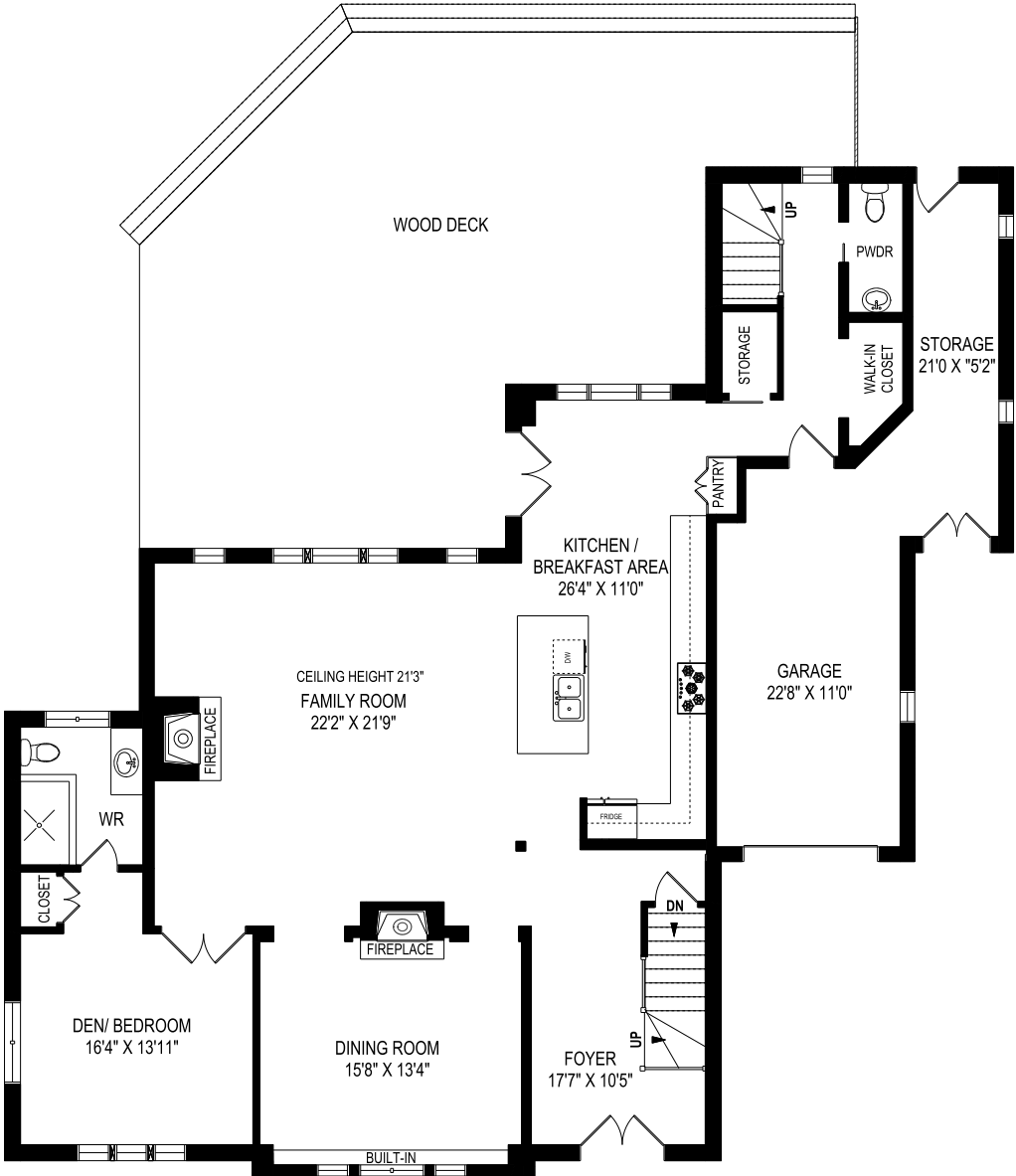
MAIN FLOOR PLAN 1848 SQUARE FEET
