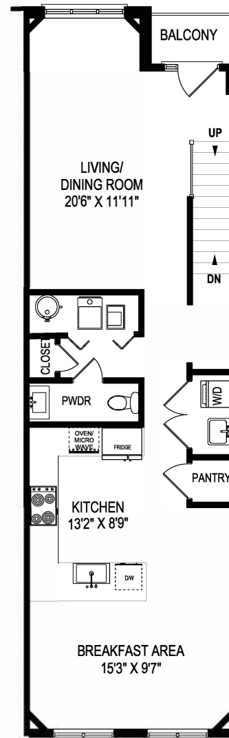
SECOND FLOOR 865 SQUARE FEET
