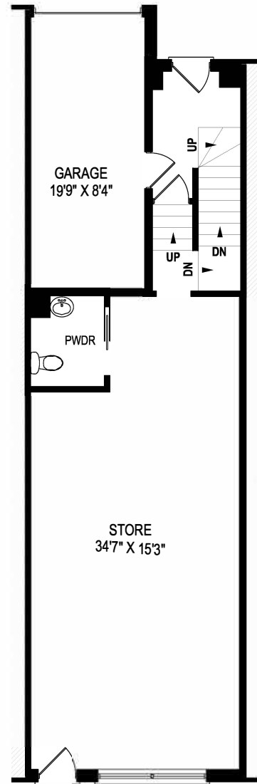
MAIN FLOOR 707 SQUARE FEET
