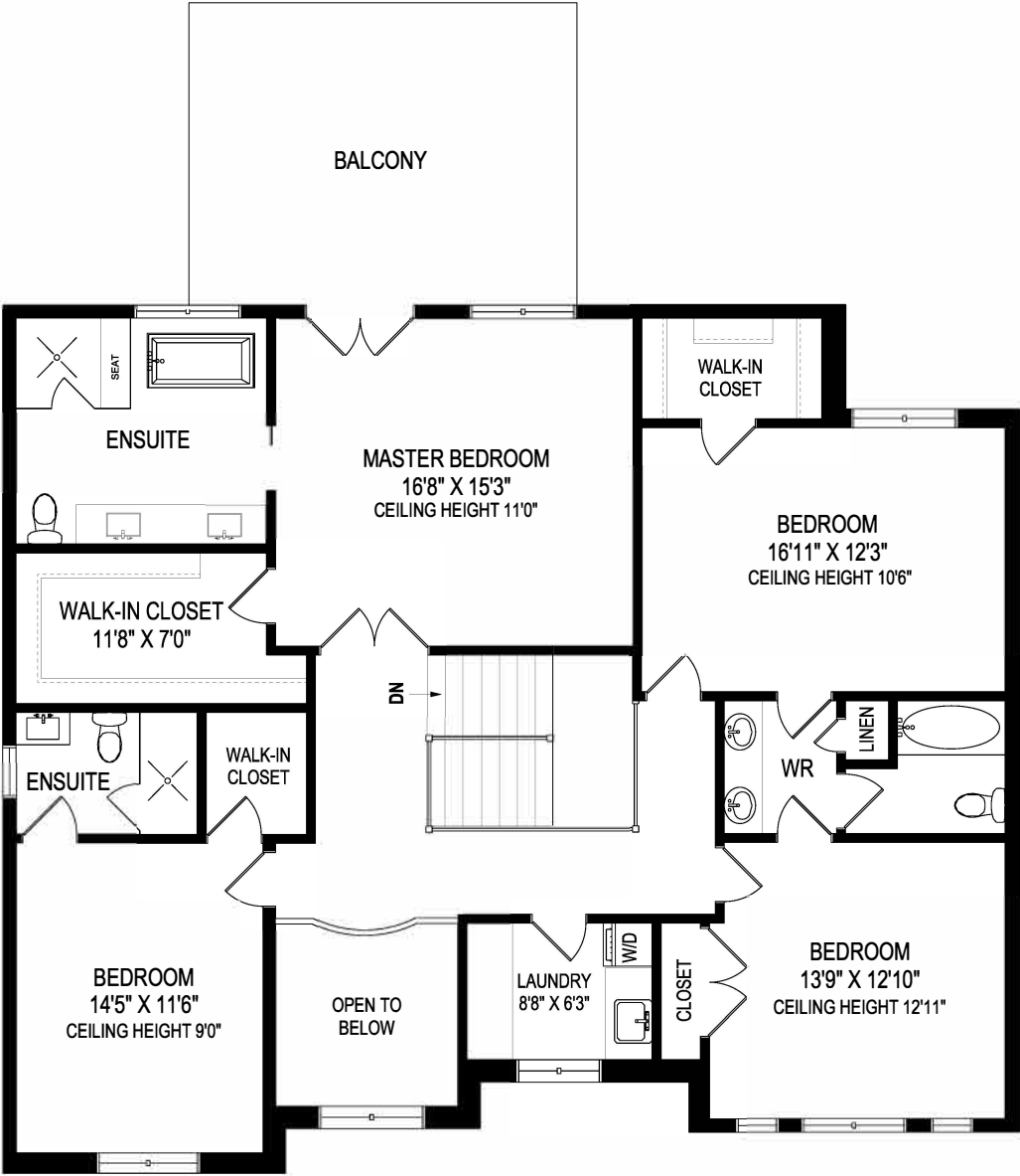
SECOND FLOOR 1717 SQUARE FEET AREA EXCLUDES 70 SQUARE FEET OPEN TO BELOW SPACE
