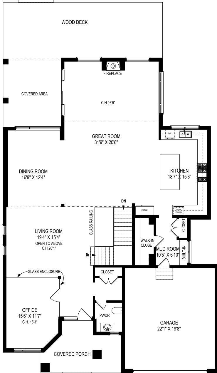
MAIN FLOOR 2091 SQUARE FEET CEILING HEIGHT 10'0"
