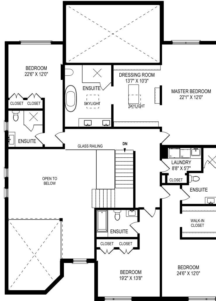
SECOND FLOOR 1916 SQUARE FEET AREA EXCLUDES 387 SQUARE FEET OPEN TO BELOW SPACE CEILING HEIGHT 9'0"
