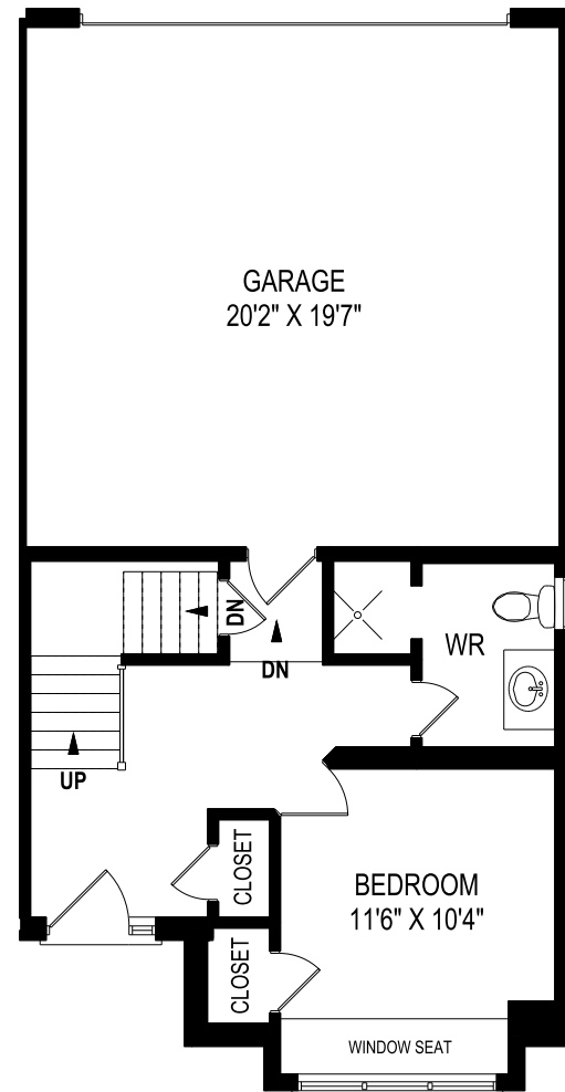
MAIN FLOOR 388 SQUARE FEET
