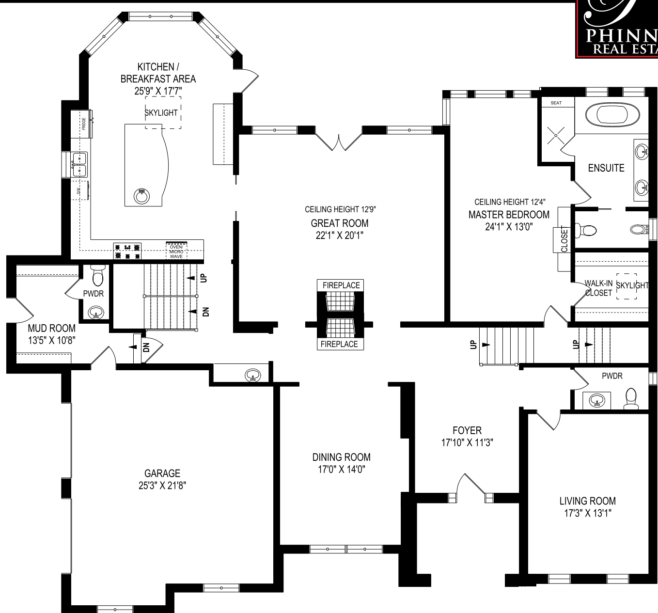
MAIN FLOOR PLAN 2857 SQUARE FEET CEILING HEIGHT 10'
