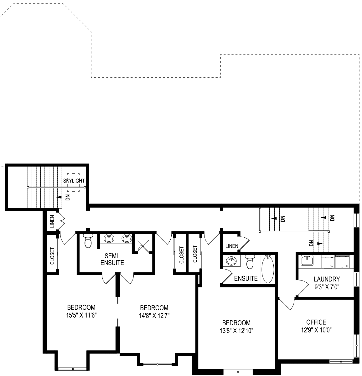
SECOND FLOOR PLAN 1518 SQUARE FEET CEILING HEIGHT 9'
