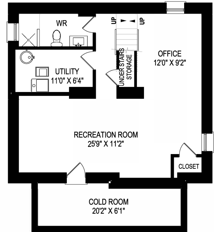
LOWER LEVEL 883 SQUARE FEET
