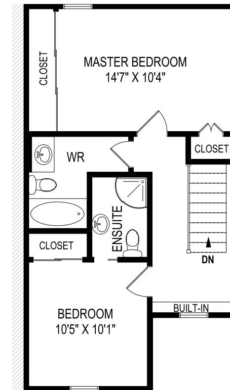
SECOND FLOOR PLAN 541 SQUARE FEET
